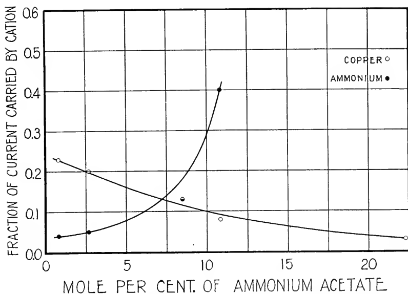
FIG. 4. Transference of copper and of ammonium in ammonium cupric acetate solutions containing 0.3 mole per cent of cupric acetate.
